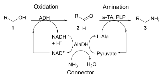
Scheme 1. Artificial redox-neutral multi-enzyme network for the bioamination of primary alcohols. ADH: alcohol dehydrogenase, ω-TA: ω-transaminase, AlaDH: L-alanine dehydrogenase, and PLP: 5'-pyridoxal phosphate.
