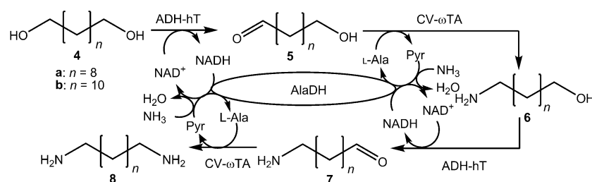
Scheme 2. Double bioamination of long-chain n -alkane-1, \omega -diols.
